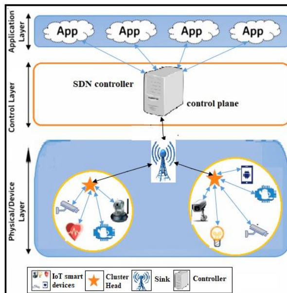
Fig.2. Network architecture for IoT devices based SDN concept
