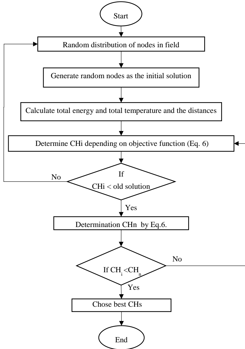
Fig.1. The flowchart of the future search algorithm
