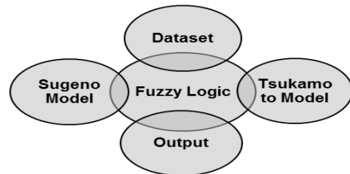
Fig.3. Framework Model
