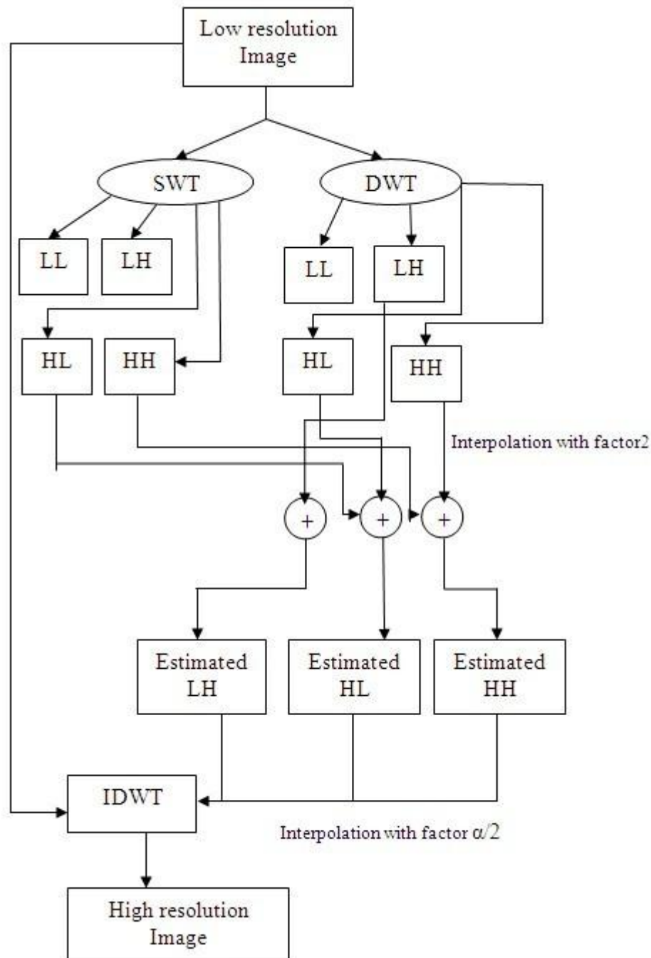
Figure-1. Block diagram of the proposed super resolution algorithm.
