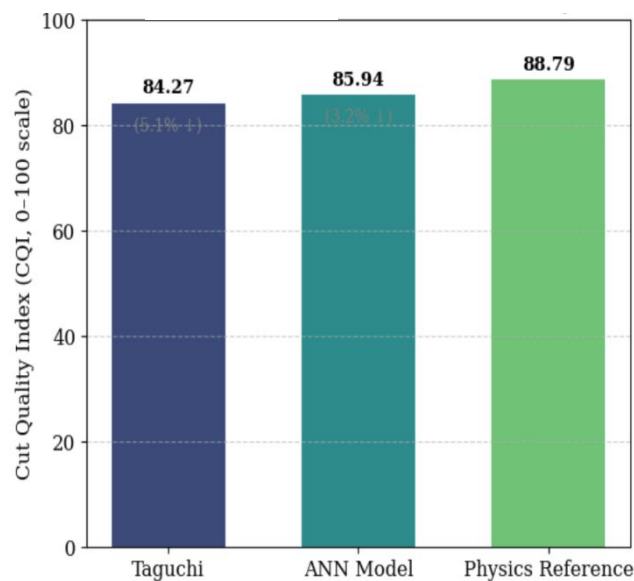
Fig. 5. Comparison of the predicted Cut Quality Index (CQI) obtained from the Taguchi method, the Artificial Neural Network (ANN) model, and the physics-calibrated digital-twin reference.
