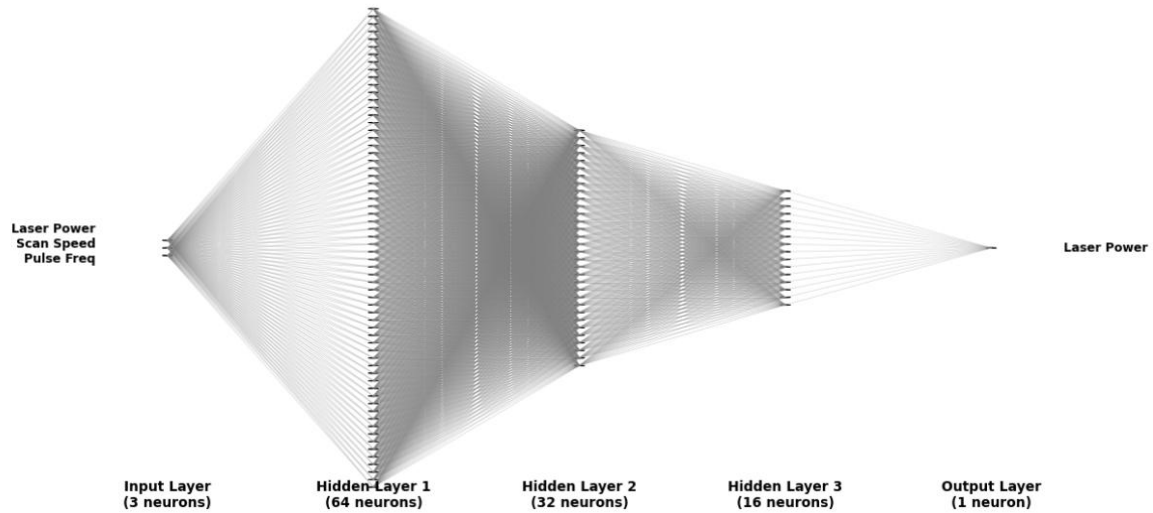
Fig. 2. Architecture of the Artificial Neural Network (ANN) model developed for predictive optimization of laser micromachining performance in stainless steel.
