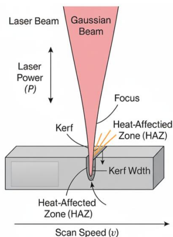
Fig. 1. presents a schematic of the fibre-laser micromachining setup used for stainless steel. A tightly focused laser beam impinges on the workpiece surface, inducing localized melting and material ejection that form a narrow kerf. The quality of this cut is governed by the interaction among laser power, scanning speed, and pulse frequency, which collectively influence the kerf geometry and the width of the heat-affected zone (HAZ).
