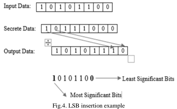
Fig.4. LSB insertion example
