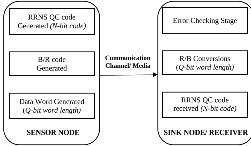
Fig. 1. General Architecture of the RNS base Wireless Sensor Networks with Error Detection
