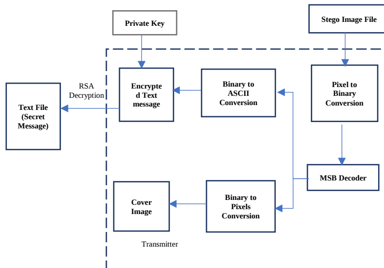
Fig. 2. Receiver section of the proposed system architecture
