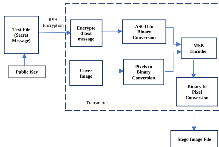
Fig. 1. Sender section of the proposed system architecture
