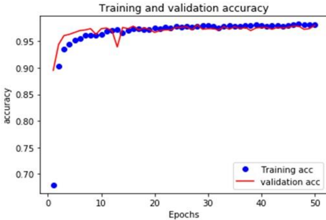
Fig. 5. Plot: Training and validation accuracy versus epochs
