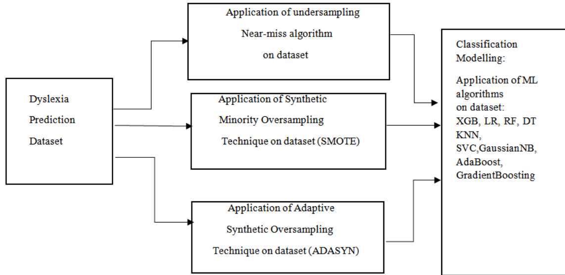
Fig. 6. Proposed Framework
