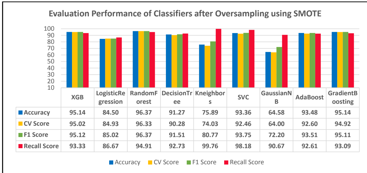
Fig.8 . Evaluation Performance of Classifiers after oversampling using SMOTE
