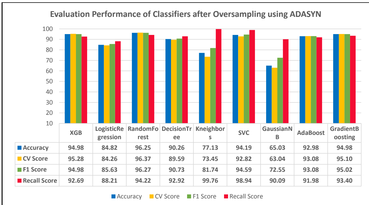
Fig.9. Evaluation Performance of Classifiers after Oversampling using ADASYN
