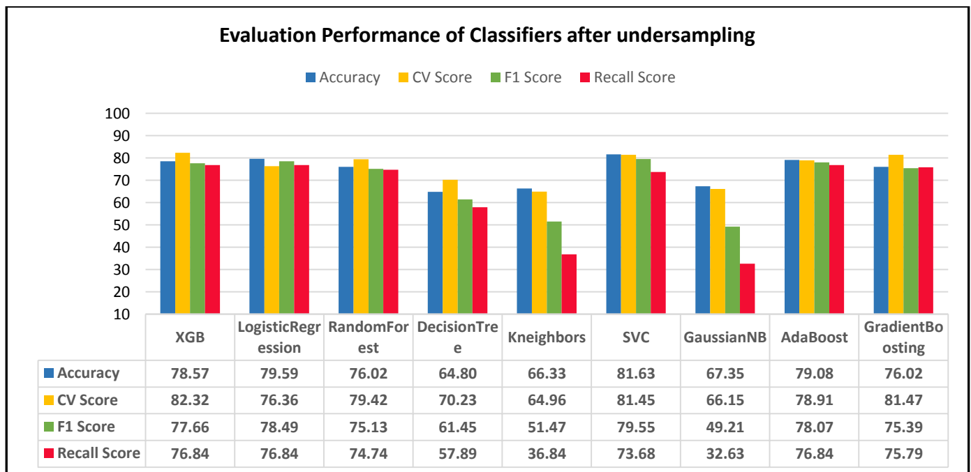
Fig.7. Evaluation Performance of classifiers after undersampling
