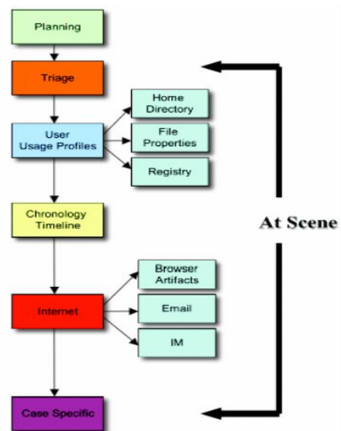
Fig. 6. Cyber Forensics Field Triage Process Model (CFFTPM) [8]
