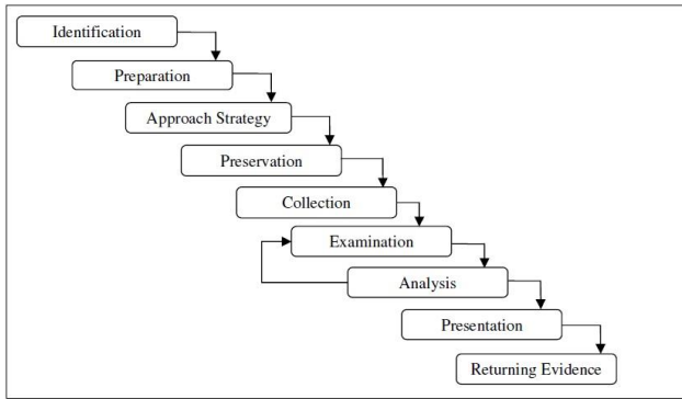
Fig. 3. Abstract Digital Forensic Model [6]
