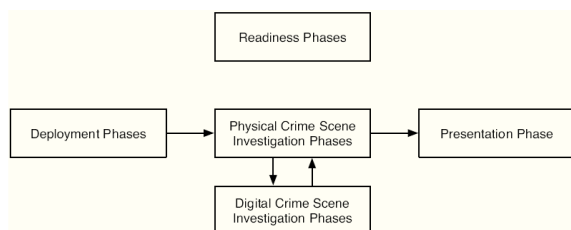
Fig. 4. Graphical Representation of IDIP Model [7]
